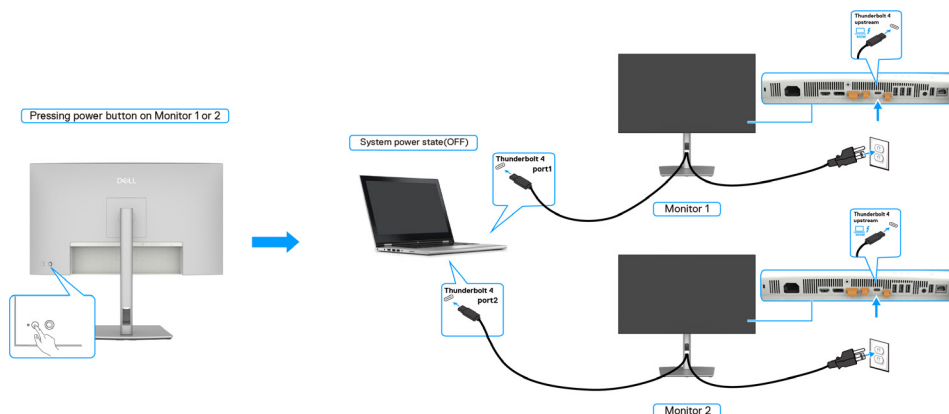
Figure 55. Pressing the power button on either monitor will turn off both monitors and the computer
