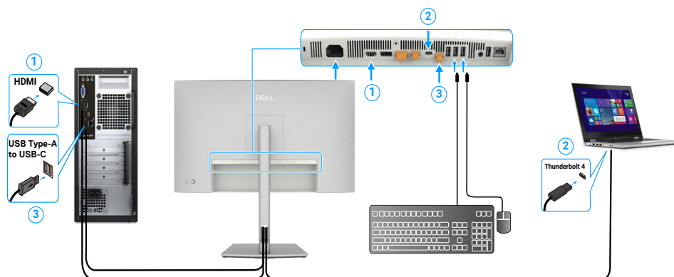
Figure 92. KVM 2 connecting
