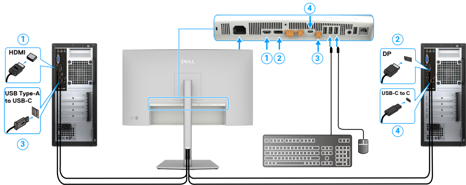
Figure 90. KVM 1 connecting
