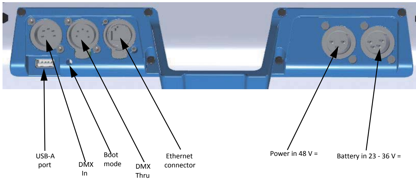
Figure 3: Connector panel
